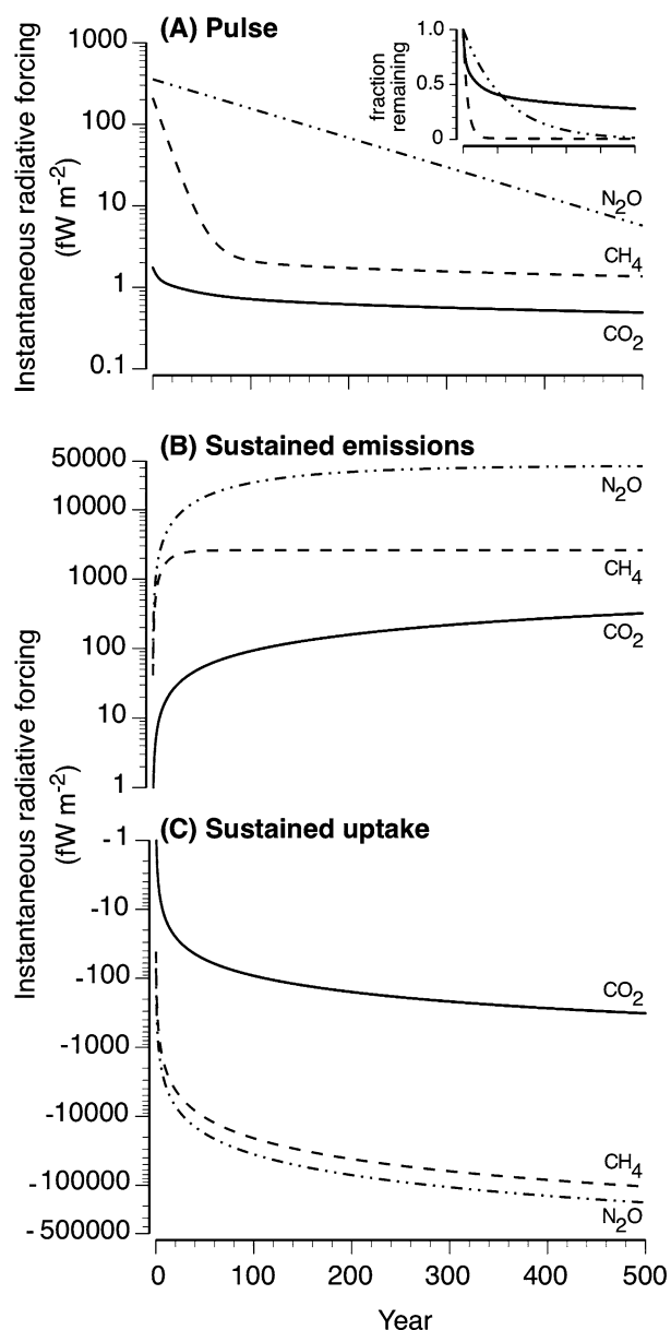
Figure 2. (A) Instantaneous radiative forcing of CO 2 , CH 4 , and N 2 O following a 1 kg pulse addition of each gas at time 0 and the decay of each gas over a 500-year period. Inset shows the fraction of each gas remaining over time. The remainder of the figure shows radiative forcing due to sustained emissions (B) or sustained uptake (C) of CO 2 , CH 4 , and N 2 O throughout the model period. All fluxes were 1 kg m -2 y -1 . In all panels, the “CH 4 ” curves include any radiative forcing by CO 2 that was produced from the oxidation of atmospheric CH 4 . Note the logarithmic scale on the y axes. fW = 10 -15 W.
