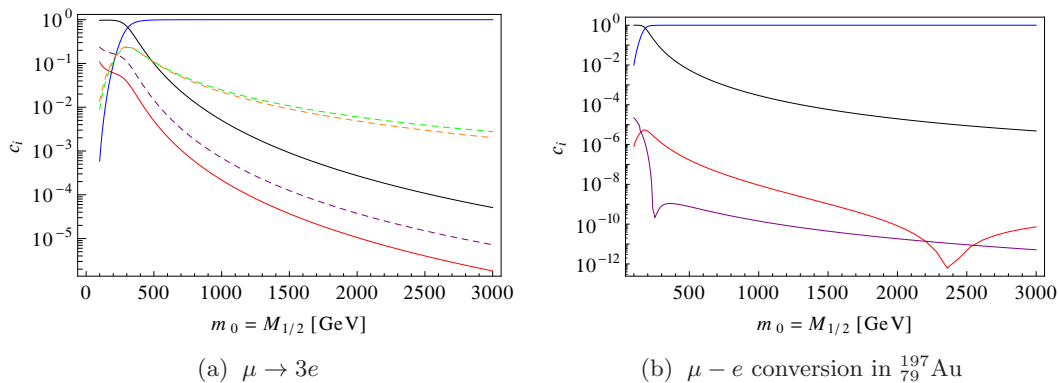
Figure 3. Relative contributions to \text{Br}(\mu \rightarrow 3e) (left-hand side) and \mu - e conversion in ^{197}\text{Au} (right-hand side) as a function of m_0 = M_{1/2} for a degenerate singlet spectrum with \hat{M}_R = 10 \text{ TeV} and M = 10^{11} \text{ GeV} . The rest of the cMSSM parameters are set to A_0 = -300 \text{ GeV} , B_0 = 0 , \tan \beta = 10 and \text{sign}(\mu) = + . On the left-hand side, solid lines represent individual contributions, \gamma (black), Z (blue) and h (red) whereas the dashed lines represent interference terms, \gamma - Z (green), \gamma - h (purple) and Z - h (orange). Note that in this case h includes both Higgs and box contributions. On the right-hand side interference terms are not shown to make the results clearer. The individual contributions are \gamma (black), Z (blue) and h (red) and boxes (purple).
