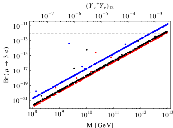
Figure 6. \text{Br}(\mu \rightarrow 3e) as a function of M and (Y_\nu^\dagger Y_\nu)_{12} for different \hat{M}_R values: \hat{M}_R = 100 \text{ GeV} (blue), \hat{M}_R = 1 \text{ TeV} (red) and \hat{M}_R = 10 \text{ TeV} (black). The cMSSM parameters are taken as in figure 5. The horizontal dashed line represents the current experimental bound.
