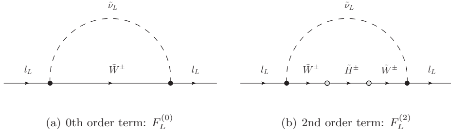
Figure 1. Diagrammatic representation of the F_L expansion in the chargino mixing angle, \theta_{\tilde{\chi}^\pm} .
