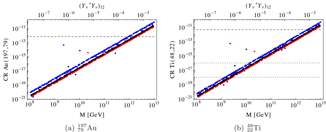
Figure 5. \mu - e conversion rates in ^{197}_{79}\text{Au} (left) and ^{48}_{22}\text{Ti} (right), as a function of M and (Y_\nu^\dagger Y_\nu)_{12} for different \hat{M}_R values: \hat{M}_R = 100 GeV (blue), \hat{M}_R = 1 TeV (red) and \hat{M}_R = 10 TeV (black). We set A_0 = -300 GeV, \tan\beta = 10 , \text{sign}(\mu) = + and B_0 = 0 , and we randomly vary m_0 and M_{1/2} in the range [0, 3 \text{ TeV}] . The horizontal dashed lines represent the current experimental bounds and the dotted ones represent the expected future sensitivities.
