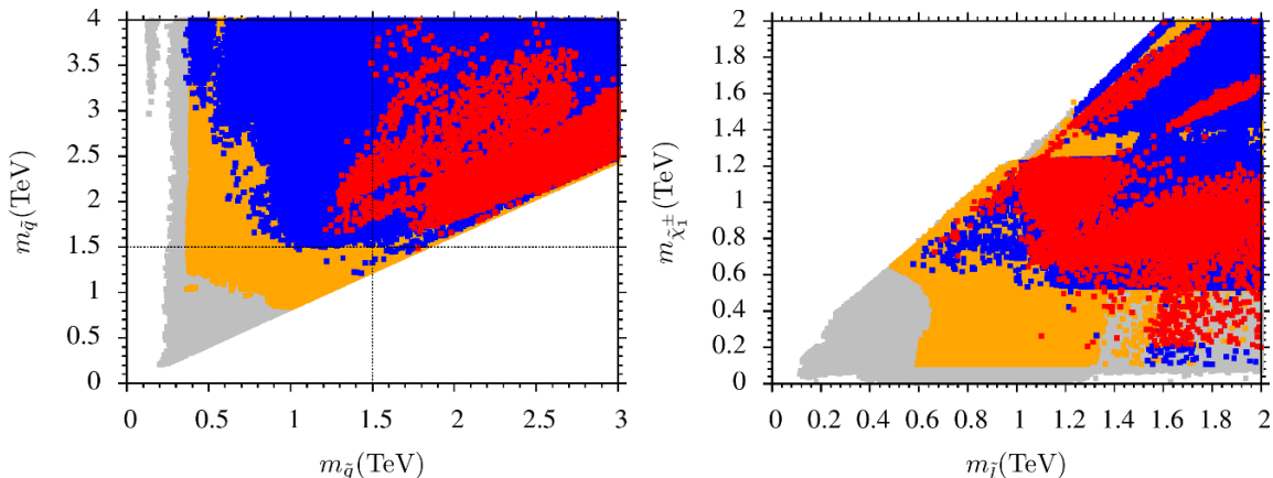
Figure 10. Plots in m_{\tilde{g}}-m_{\tilde{q}} and m_{\tilde{t}}-m_{\tilde{\chi}_1^\pm} planes for NUHM2. In the left panel orange points do not satisfy gluino and first two generation squark mass bounds and red points are a subset of blue point solutions and also satisfy bounds for neutralino relic abundance, 0.001 \leq \Omega h^2 \leq 1 . Dashed vertical and horizontal lines stand for current squark and gluino lower mass bounds respectively. Otherwise color coding is the same as in figure 2.
