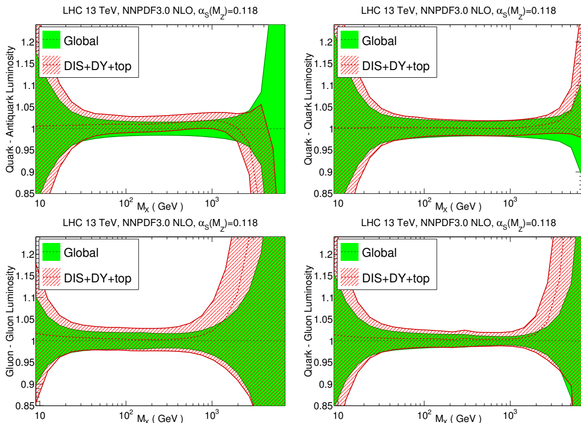
Figure 12. Comparison of the NNP3.0 NLO partonic luminosities for \alpha_s(m_Z^2) = 0.118 , in the global fit and in the DIS+DY+top fit which is used as fixed-order baseline for the resummed fits. In the upper plots we show the quark-antiquark and quark-quark luminosities, and in the lower plots the gluon-gluon and gluon quark luminosities. The calculation has been performed for the LHC 13 TeV, as a function of the mass of the final state M_X , and results are normalised to the central value of the global fit.
