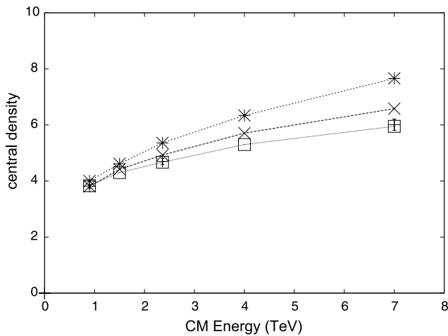
Fig. 1 The central density in pseudorapidity for the ALICE pp data (crosses with error bars), PYTHIA 8.107 ( \times signs), PYTHIA 8.135 default (asterisks) and PYTHIA 8.135 tuned (squares) as a function of the CM energy. The model prediction points are connected by lines to guide the eye
