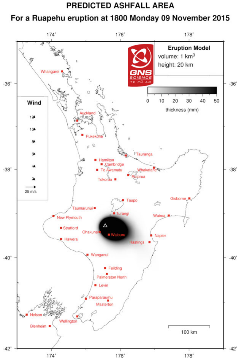
Fig. 4 Example of automatically-generated map for Ruapehu volcano for 1800 Monday 09 November 2015, showing predicted ashfall extent for one of nine pre-calculated scenarios (1 km 3 eruption volume, 20 km plume height)
