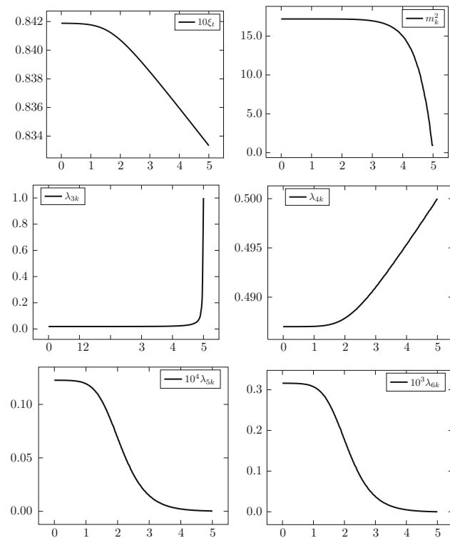
Fig. 4 Running of the non-minimal parameter \xi_t and couplings m_k^2, \lambda_{3k}, \dots, \lambda_{6k} (in units of \mu ) as functions of t = \log(k/\mu) . The initial data at the cutoff scale k = \Lambda = \mu e^5 are m^2 = \mu^2, \lambda_4 = 0.5, \lambda_3 = \mu, \lambda_5 = \lambda_6 = 0 , and \xi = 1/6
