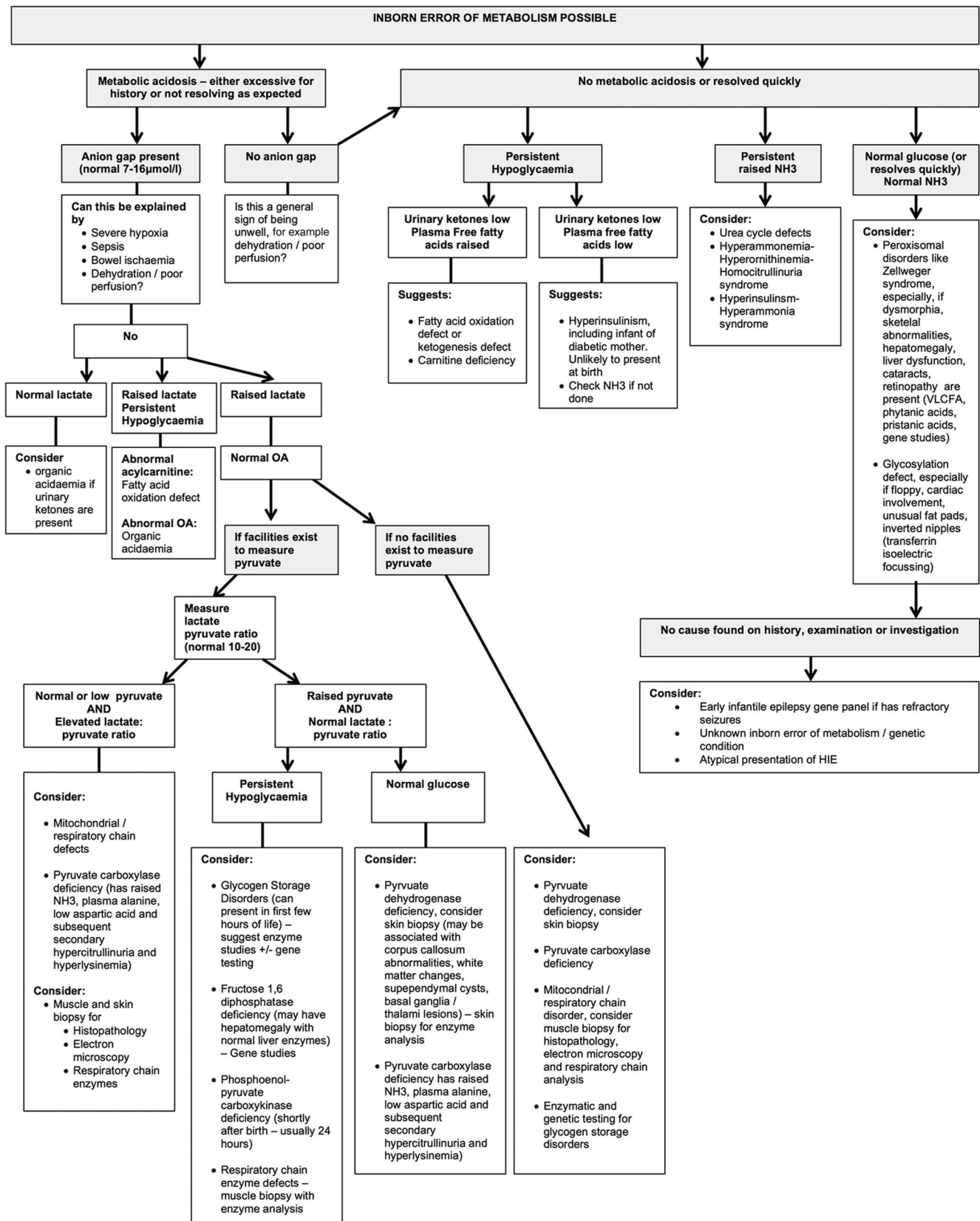
Figure 1 Flow chart to help to determine the cause of neonatal encephalopathy where the history and courses are not typical of hypoxia ischaemia. aAASA, alpha amino adipic semialdehyde; aEEG, amplitude integrated EEG; CK, creatine kinase; CSF, cerebrospinal fluid; cUSS, cranial ultrasound scan; DCT, direct Coombs test; EEG, electroencephalogram; EMG; electromyography; FH, family history; FBC, full blood count; GABA, Gaba-aminobutyric acid; HIE, hypoxic-ischaemic encephalopathy; LFT, liver function test; IV, intravenous; NH3, ammonia; OA, organic acids; U&E, urea and electrolytes; WBC, white blood cell count; VLCFA, very long chain fatty acids.
