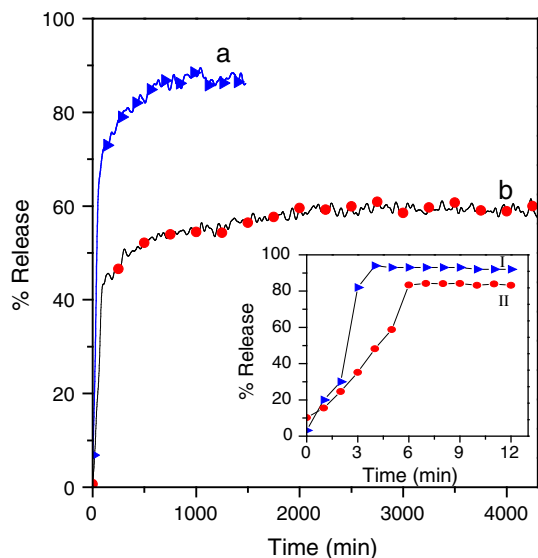
Fig. 6 Release profiles of PE from the FPEGPE nanocomposite into (a) phosphate buffered solution at pH 4.8 and (b) pH 7.4. The inset shows the release profiles of PE from its physical mixture of FNPs–PEG–PE into phosphate buffered solution (I) at pH 4.8 and (II) at pH 7.4
