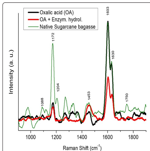
Figure 5 Raman spectra of native sugarcane bagasse (green online), pre-treated bagasse with oxalic acid (black online) and oxalic acid hydrolysis pre-treated bagasse (red line). A gradual reduction in band intensities was recorded in OAFEX and enzymatic hydrolysis revealing the displacement in hemicellulose backbone and enzymatic cleavage of \beta -1-4-glycosidic linkage in cellulose.
