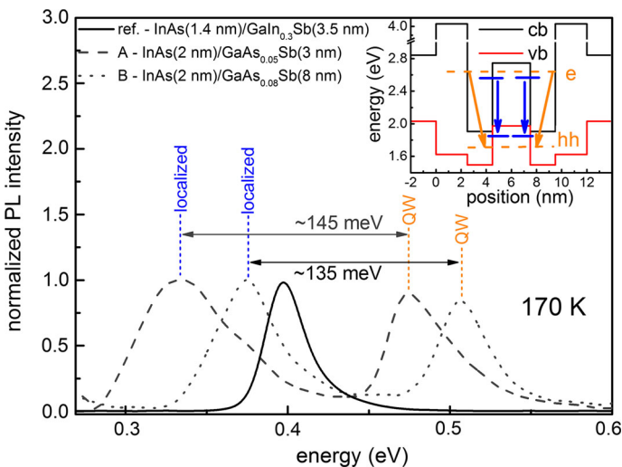
Fig. 1 Photoluminescence spectra for the reference InAs/GaInSb sample (solid) and two samples with GaAsSb layer of different thickness and As content (see legend). (inset) Band alignment: cb and vb stand for conduction band edge and valence band edge, respectively. Orange and blue arrows indicate the QW and localized transitions
