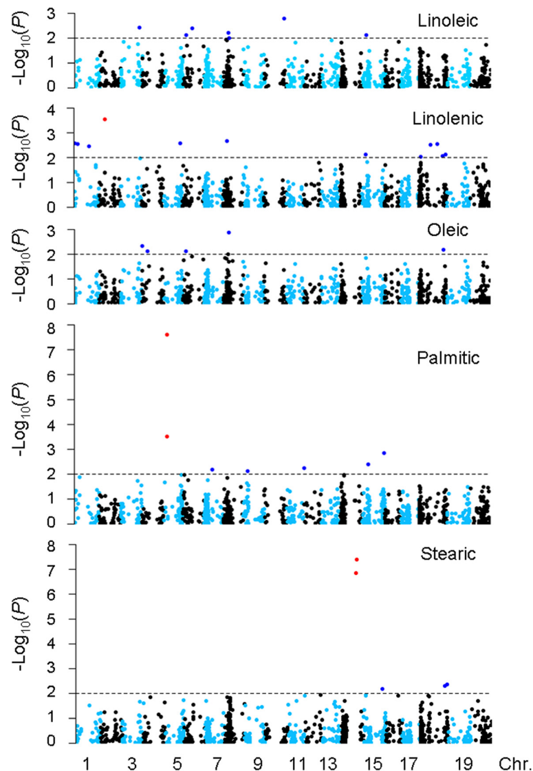
Fig. 4 Manhattan plots of p values indicating SNP markers associated with five fatty acids. The x- axis shows SNP markers along each soybean chromosome; y- axis is the -\log_{10}(p) value, horizontal lines designate 1E-02 thresholds for significant associations. The association of SNP markers with highly significant associations ( p < 0.001 ) are shown by red dots
