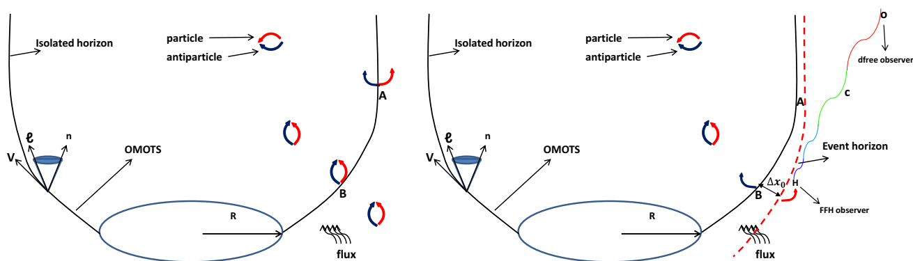
Fig. 1 On the left hand Particle creation without the UP. On the right Particle creation considering the UP. The OMOTS (outer marginally trapped 3-surface) is the same apparent horizon in both figures
