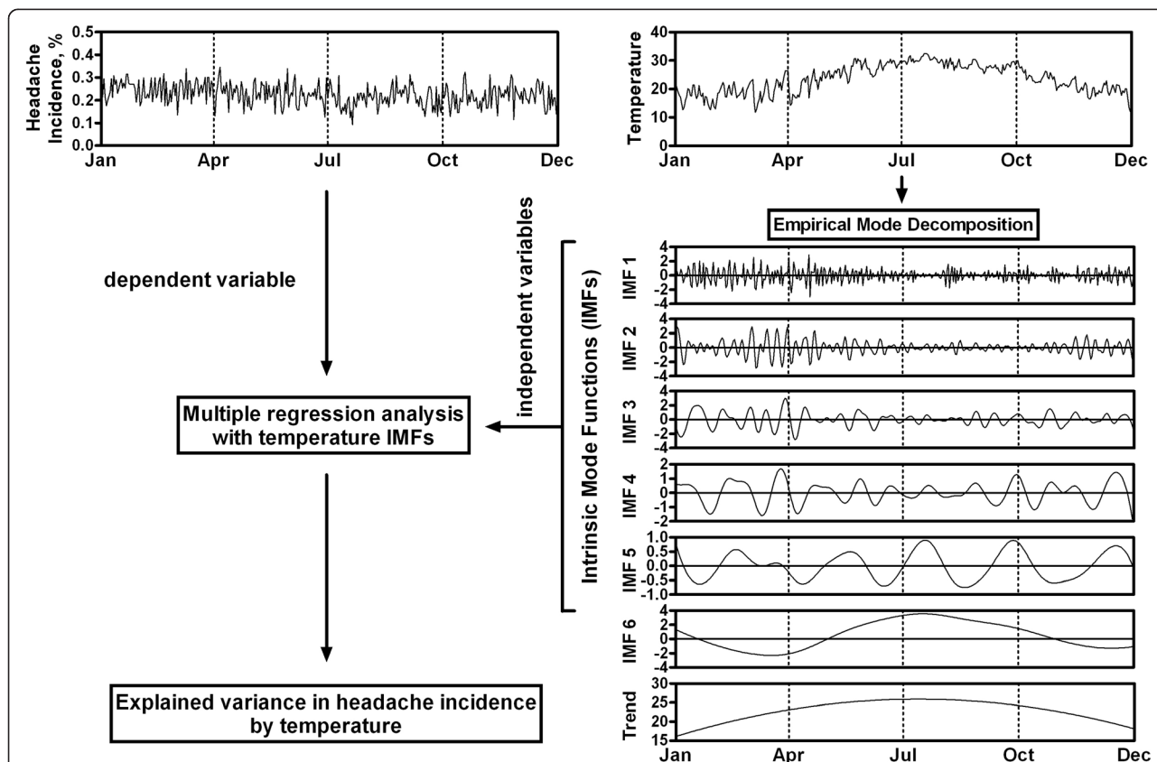
Fig. 1 Flow chart of time series analysis of headache and temperature data. Using empirical mode decomposition method, temperature time series was decomposed into an overall trend and various modes of fluctuations, termed intrinsic mode functions (IMFs). Each IMF represents a specific mode of temperature fluctuations. These IMFs were correlated with headache incidence data by multiple regression analysis to derive the explained variance in headache incidence by temperature
