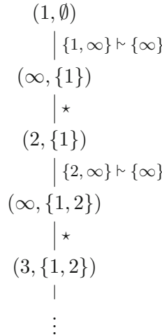
Figure 2. Counterexample to (Or^\infty)
