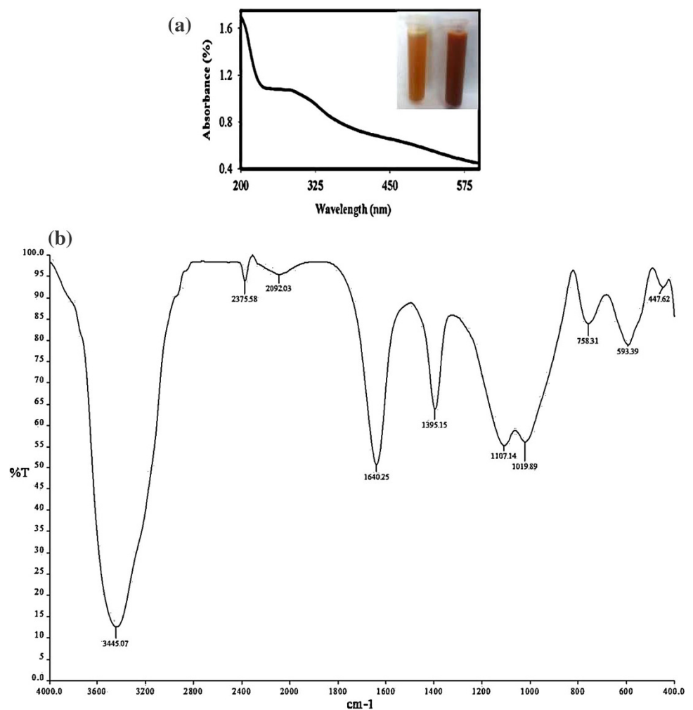
Fig. 1 a UV–Vis spectra of colloidal titanium dioxide nanoparticles synthesized using Azadirachta indica ; b Fourier transform infrared spectra of titanium dioxide nanoparticles
