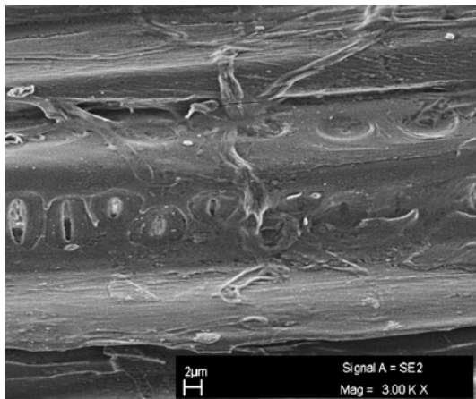
Fig. 12 Radial section of untreated beech wood after 24 months of outside exposure, 3000×
