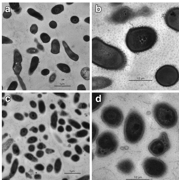
Fig. 3 Electron microscopy demonstrating antimicrobial effect of resveratrol. Electron microscopy images of P. acnes left untreated ( a, b ) or incubated for 24 h ( c, d ) with resveratrol. Images were taken at \times 10,000 magnification ( a, c ) or \times 29,000 magnification ( b, d ). Scale bar is 1 \mu\text{m} ( a, c ) or 1/2 \mu\text{m} ( b, d )
