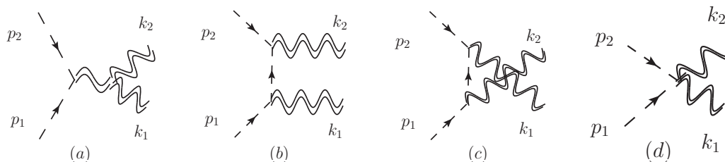
Figure 1. The various contributions to the tree-amplitude \phi + \phi \rightarrow 2 gravitons: (a) s -channel, (b) t -channel, (c) u -channel, (d) contact term.
