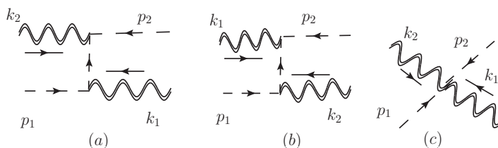
Figure 2. Compton scattering given by the t -channel contribution in (a), the u -channel contribution in (b) and the contact term in (c).
