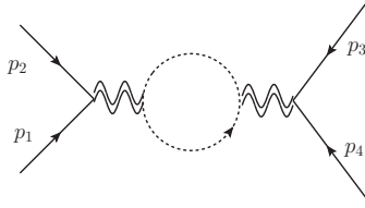
Figure 4. The ghost contribution from the vacuum polarization of the graviton
