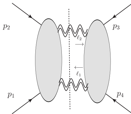
Figure 3. The cut considered. The loop momenta are flowing clockwise. And the on-shell conditions are \ell_1^2 = 0 and \ell_2^2 = (\ell_1 + p_1 + p_2)^2 = 0 . Solid lines are massive and wiggly lines are massless.
