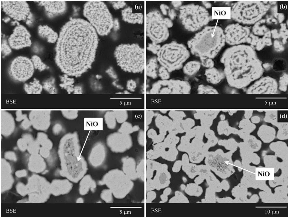
Fig. 15—Backscattered electron images showing internal microstructures of BNC reduced in 1.5 pct H_2-N_2 ; heating rate 10\text{ }^\circ\text{C}/\text{min} at various temperatures: (a) 600\text{ }^\circ\text{C} , (b) 700\text{ }^\circ\text{C} , (c) 800\text{ }^\circ\text{C} , and (d) 900\text{ }^\circ\text{C} . The gray phases are the residual nickel oxide.
