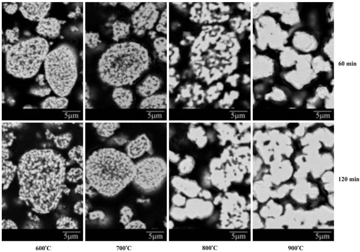
Fig. 9—SEM micrographs of the cross sections of BNC samples reduced in 15 pct H_2-N_2 at 60 and 120 min (10 °C/min heating rate) at various temperatures, showing extensive densification at temperatures above 700 °C.
