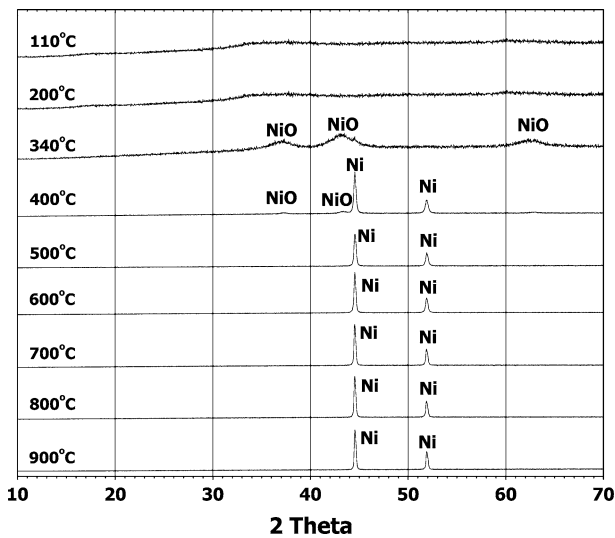
Fig. 7—XRD spectra of BNC sample reduced in 15 pct H 2 -N 2 at various temperatures. Heating rate 10 °C/min, holding time at temperature 30 minutes, Cu K α radiation used.
