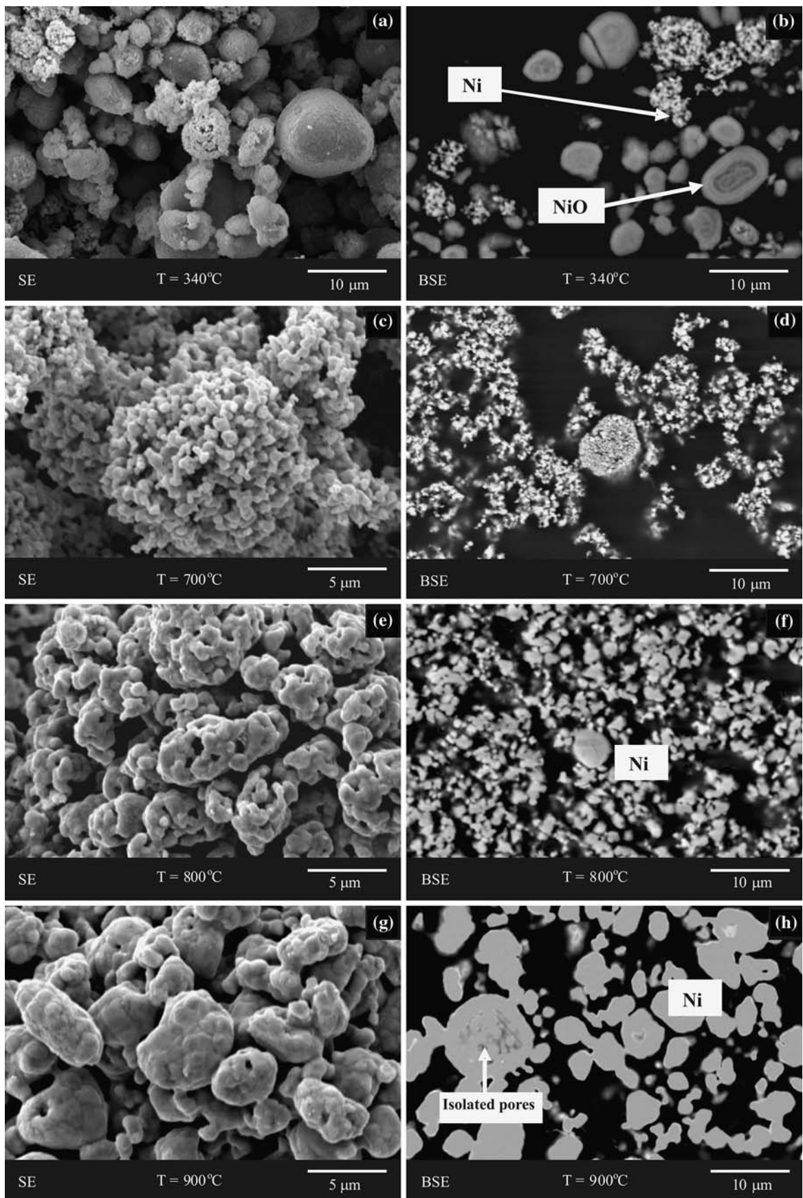
Fig. 8—SEM micrographs of the surface (left column) and the sections (right column) of BNC sample reduced in 15 pct H_2-N_2 (30 min, 10 °C/min heating rate) at various temperatures: (a) and (b) 340 °C, (c) and (d) 700 °C, (e) and (f) 800 °C, and (g) and (h) 900 °C. Nickel metal appears as the bright phase in (b).
