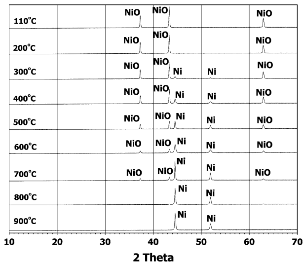
Fig. 11—XRD spectra of the preoxidized BNC samples in air at 900 °C (30 min, 10 °C/min heating rate), which were then reduced in 15 pct H 2 -N 2 (30 min, 10 °C/min heating rate) at various fixed temperatures; Cu K α radiation is used.
