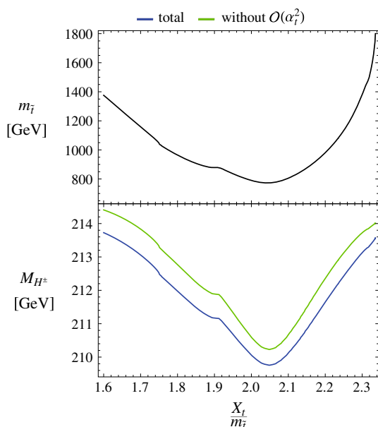
Fig. 5 Mass M_{H^\pm} of the charged Higgs boson with all available higher-order terms and without the \mathcal{O}(\alpha_t^2) contributions, for ranges of m_{\tilde{t}_1} and X_t allowed by HiggsBounds and m_h = 125 GeV. Other parameters are m_A = 200 GeV, \tan\beta = 8 , \mu = 3000 GeV, A_b = A_\tau = 0 , m_{\tilde{g}} = 1000 GeV, m_{\tilde{g}} = 1500 GeV
