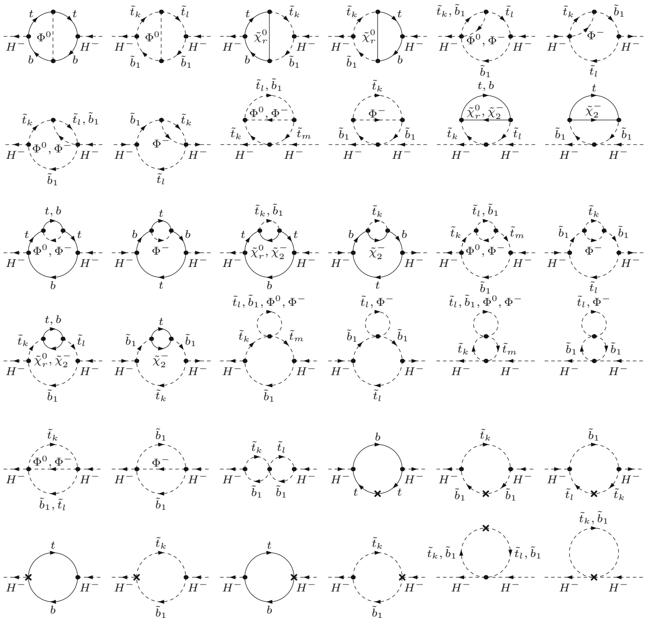
Fig. 1 Full list of two-loop self-energy diagrams for the charged Higgs bosons. Each cross denotes a one-loop counterterm insertion. \Phi^0 = h, H, A, G ; \Phi^- = H^-, G^-
