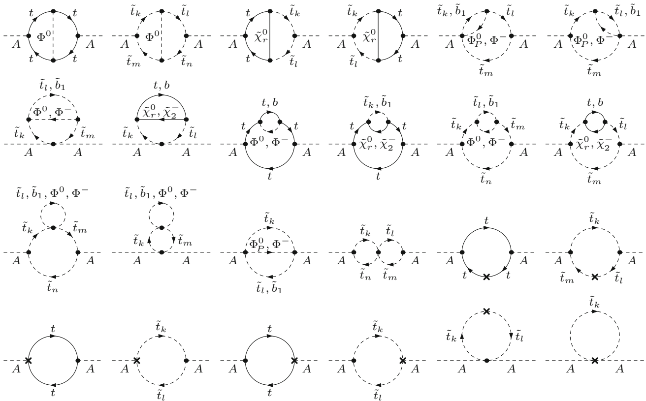
Fig. 2 Full list of two-loop self-energy diagrams for the A-boson. Each cross denotes a one-loop counterterm insertion. \Phi^0 = h, H, A, G ; \Phi_P^0 = A, G ; \Phi^- = H^-, G^-
