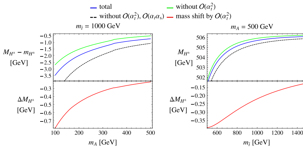
Fig. 3 Upper parts: prediction for the charged Higgs-boson mass M_{H^\pm} including all known contributions (blue), without the \mathcal{O}(\alpha_t^2) contributions (green) and without any two-loop corrections (black dashed) [ m_{H^\pm} is the tree-level mass according to Eq. (2.6)]. Lower parts the
