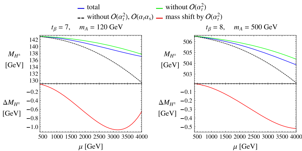
Fig. 4 Upper parts prediction for the charged Higgs-boson mass M_{H^\pm} including all known contributions (blue), without the \mathcal{O}(\alpha_t^2) contributions (green) and without any two-loop corrections (black dashed). Lower parts the mass shift \Delta M_{H^\pm} by the \mathcal{O}(\alpha_t^2) contributions (red).
