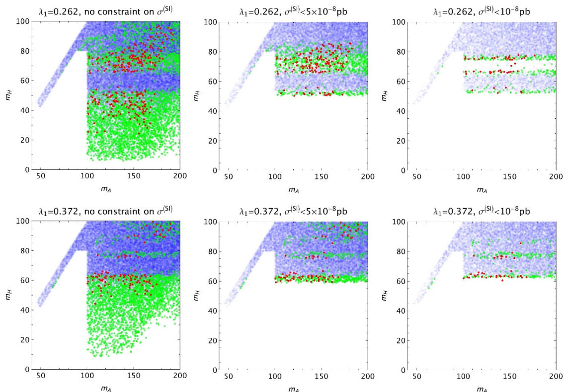
Figure 7. Left: parameter region (m_{A^0}, m_{H^0}) consistent with collider/electroweak precision constraints and dark matter relic density. Middle: left + direct detection with \sigma^{(SI)} < 5 \times 10^{-8} \text{pb} . Right: left + direct detection with \sigma^{(SI)} < 10^{-8} \text{pb} . In each panel, the parameter space satisfying (0.094 <) \Omega_{\text{DM}} h^2 < 0.136 is in blue (green) and the region allowed by the pure SM Higgs inflation in addition to 0.094 < \Omega_{\text{DM}} h^2 < 0.136 is in red. In the upper (lower) row, we set \lambda_1 = 0.262 ( \lambda_1 = 0.372 ), which corresponds to m_h = 126 \text{ GeV} ( m_h = 150 \text{ GeV} ).
