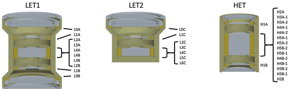
Fig. 29 Cut-away illustration of the EPI-Hi telescope designs and detector naming
