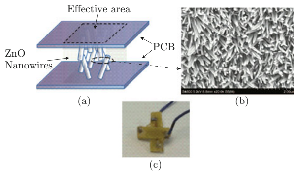
Fig. 1 (a) Schematic graph of the device (effective area is around 1000 \mu\text{m} \times 1000 \mu\text{m} ); (b) Scanning electron photograph of ZnO nanowires on copper; (c) Photograph of a fabricated device.
