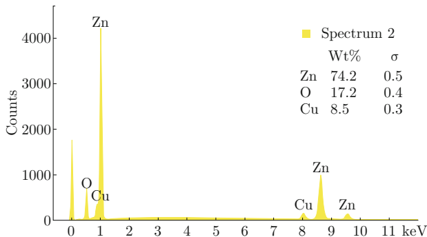
Fig. 2 Energy dispersive X-ray result showing elements distributions in the ZnO nanowires.
