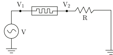
Fig. 3 Circuit diagram shows how I-V curve of the device was characterized.
