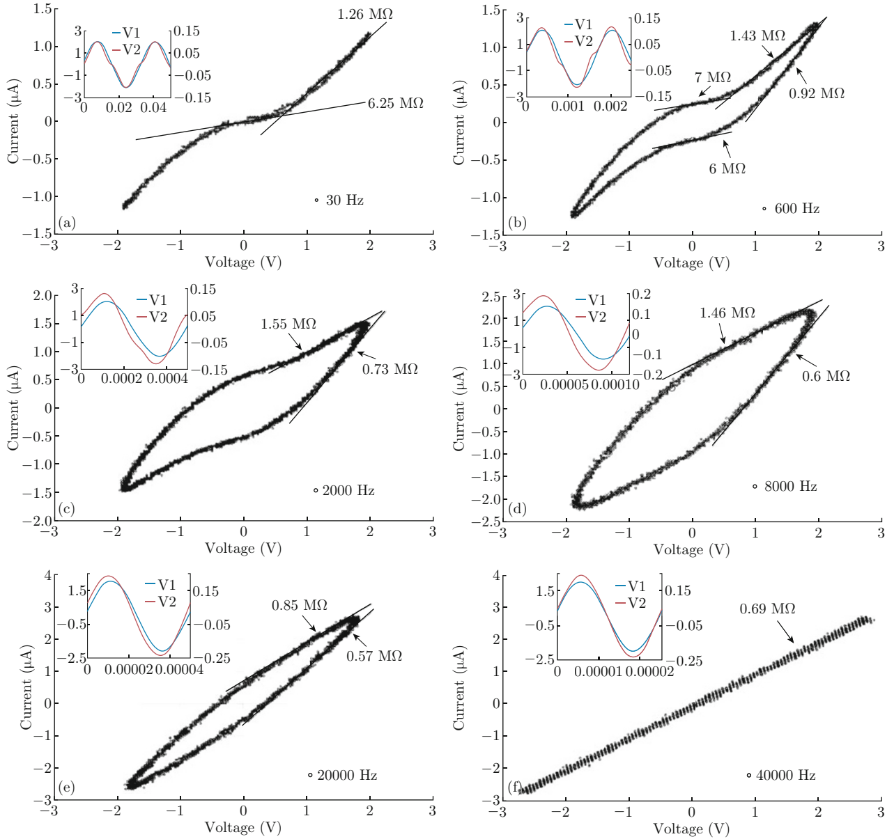
Fig. 4 I - V testing of the device. The frequency of the external source varies from 30 Hz to 40 kHz, giving different I - V characteristics.
