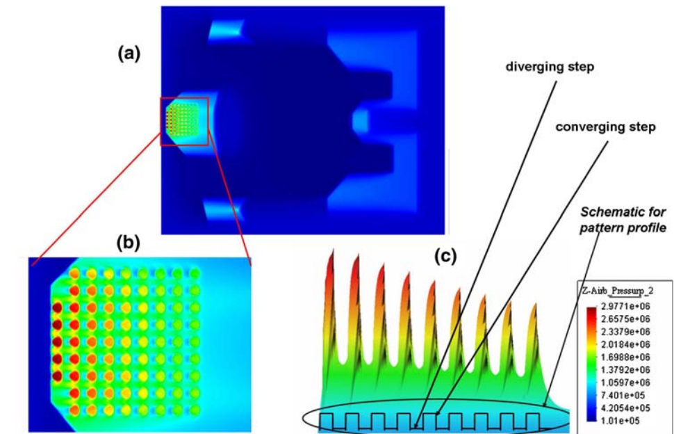
Fig. 4 Steady state pressure distribution for: a patterned air bearing slider, b zoom in plot for pressure on the center trailing pad with pattern, c side view along the slider centerline
