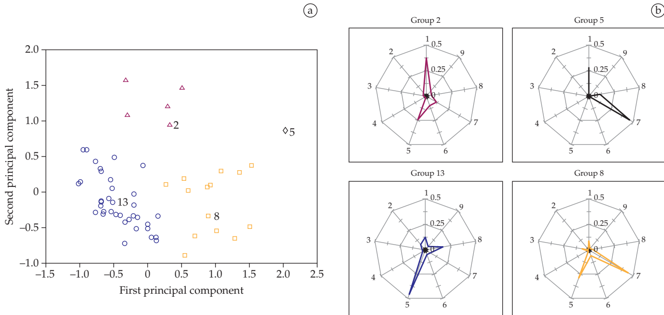
Figure 6. Analysis of the scientific productions profile: a) Clustering of 56 research groups in Computer Science associated to the São Paulo State. Note that four classes were identified. Each class is represented by a different geometric form. b) Radar charts of representative groups of the identified classes. The axes, represented by a number, are related to each type of production listed in Figure 5a.
