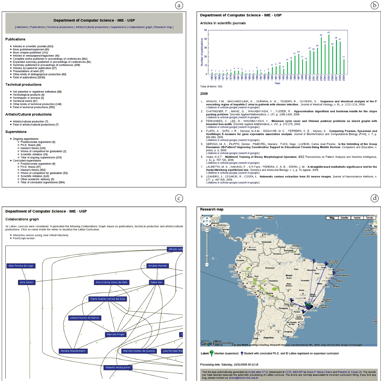
Figure 3. An example of reports obtained with scriptLattes: a) Index of generated pages; b) List of articles in scientific journals; c) Collaboration graph; (d) Research map. These results are available at http://www.vision.ime.usp.br/creativision/publications_dcc/ .
