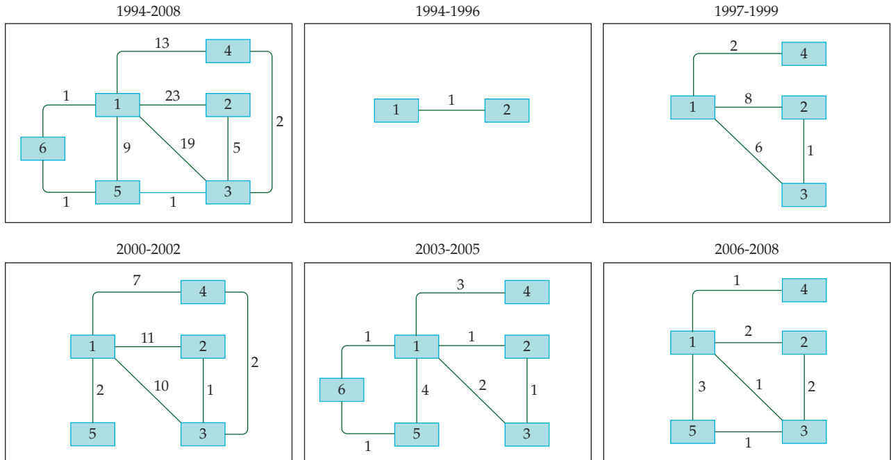
Figure 4. Temporal graph of collaborations based on the productions belonging to the Computer Vision Research Group 24 of the Department of Computer Science at University of São Paulo. The edge weight represents the number of co-authored productions.
