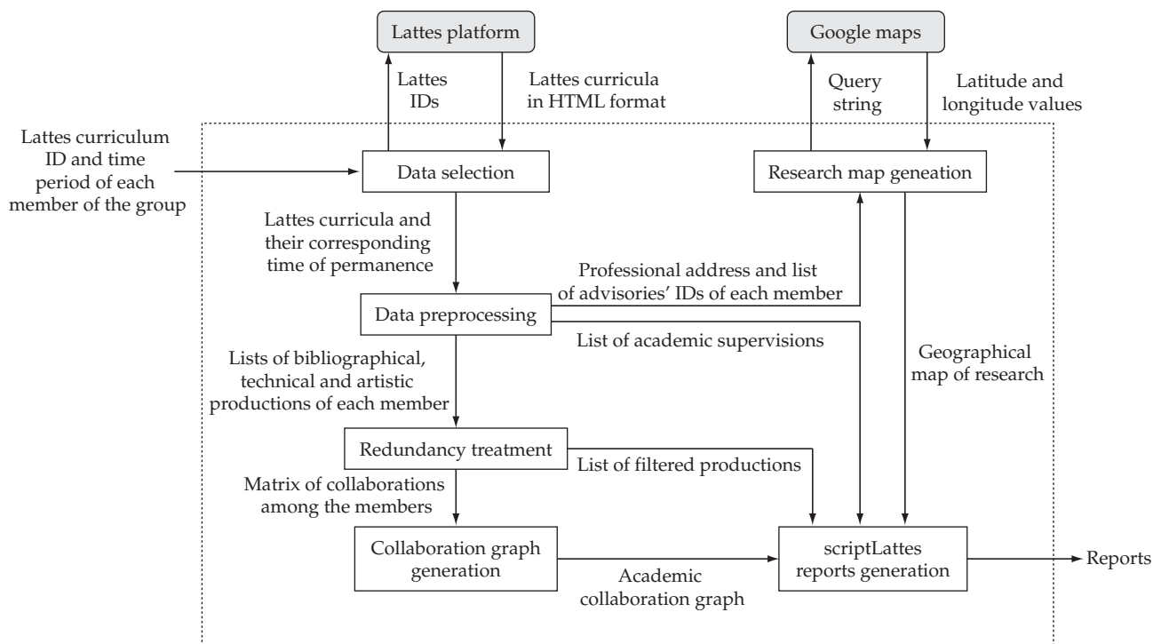
Figure 2. Schematic data flow diagram of the system (dotted lines). Each block (solid lines) represents a module while each arrow represents the information flow between modules or external platforms (gray boxes).
