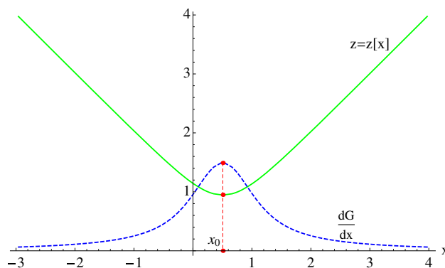
Fig. 1 Plot of z(x) and dG/dx (with r_c = 1 ). The wormhole throat is at the minimum of z(x) (maximum of G_x )
