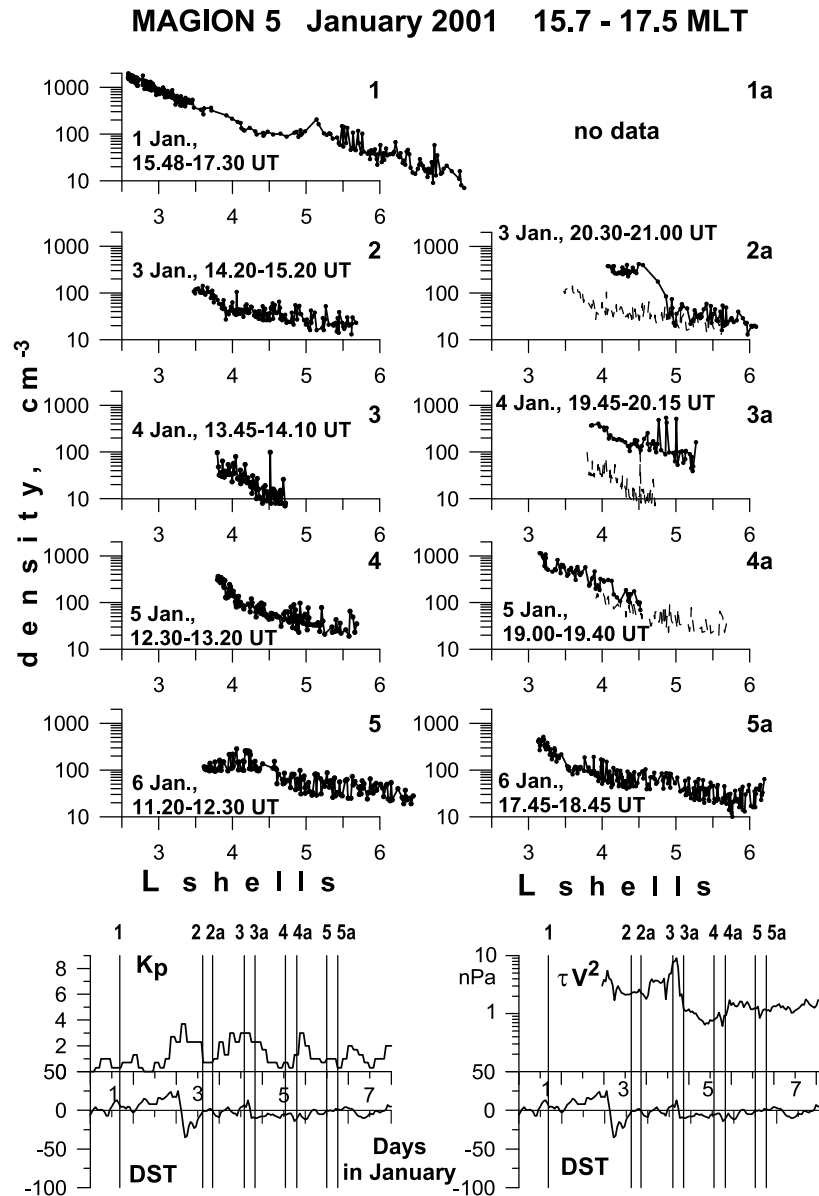
Fig. 5. Density versus L profiles measured at 15.7–17.5 MLT in successive inbound plasmasphere passes during 1–6 January 2001. Bottom plots present K_p and Dst variations during the same time period, \rho V^2 values give the solar wind dynamic pressure measured by the ACE spacecraft and shifted to the Earth ( http://cdaweb.gsfc.nasa.gov/ ). Dashed profiles in panels 2a, 3a, and 4a repeat the profiles in panels 2, 3, 4 respectively.
