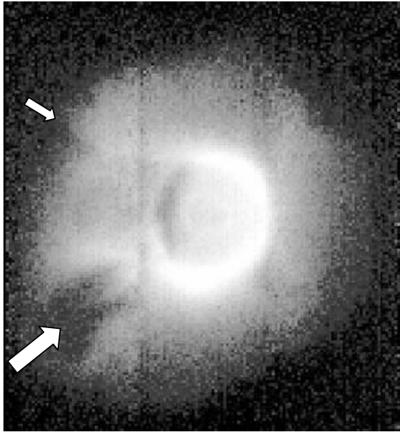
Fig. 6(a). EUV image showing the distribution of He + in the Earth's plasmasphere obtained at 17.12 UT on 24 June 2000. The sun is to the right. Big arrow marks the notch region, small arrow pointed to the shoulder.
