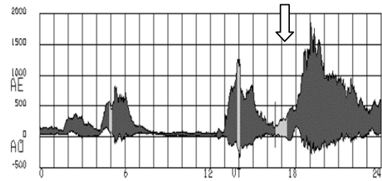
Fig. 6(c). Variations of AE and AQ indices on 23 June 2000. The arrow marks the time a day before the IMAGE measurements shown in Fig. 3.
