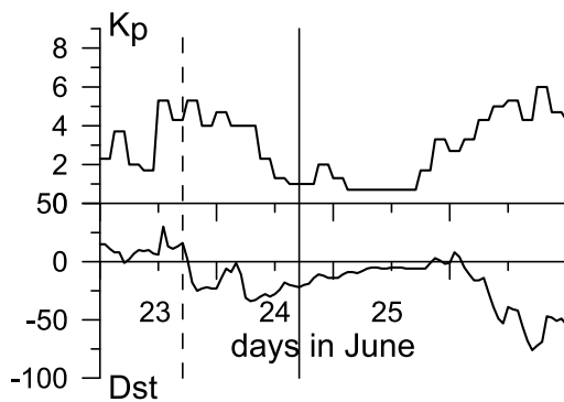
Fig. 6(b). Variations of K p and Dst indices during 23–26 June 2000. Vertical solid line marks the times of IMAGE measurements shown in Fig. 3. Dashed line marks the same hour a day before.
