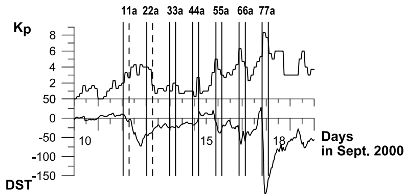
Fig. 3(b). Variations of K_p and Dst indices during 12–18 September 2000. Vertical solid lines mark the times of measurements for profiles shown in Fig. 2. (Dashed lines mark the times of orbits when no data were obtained.)
