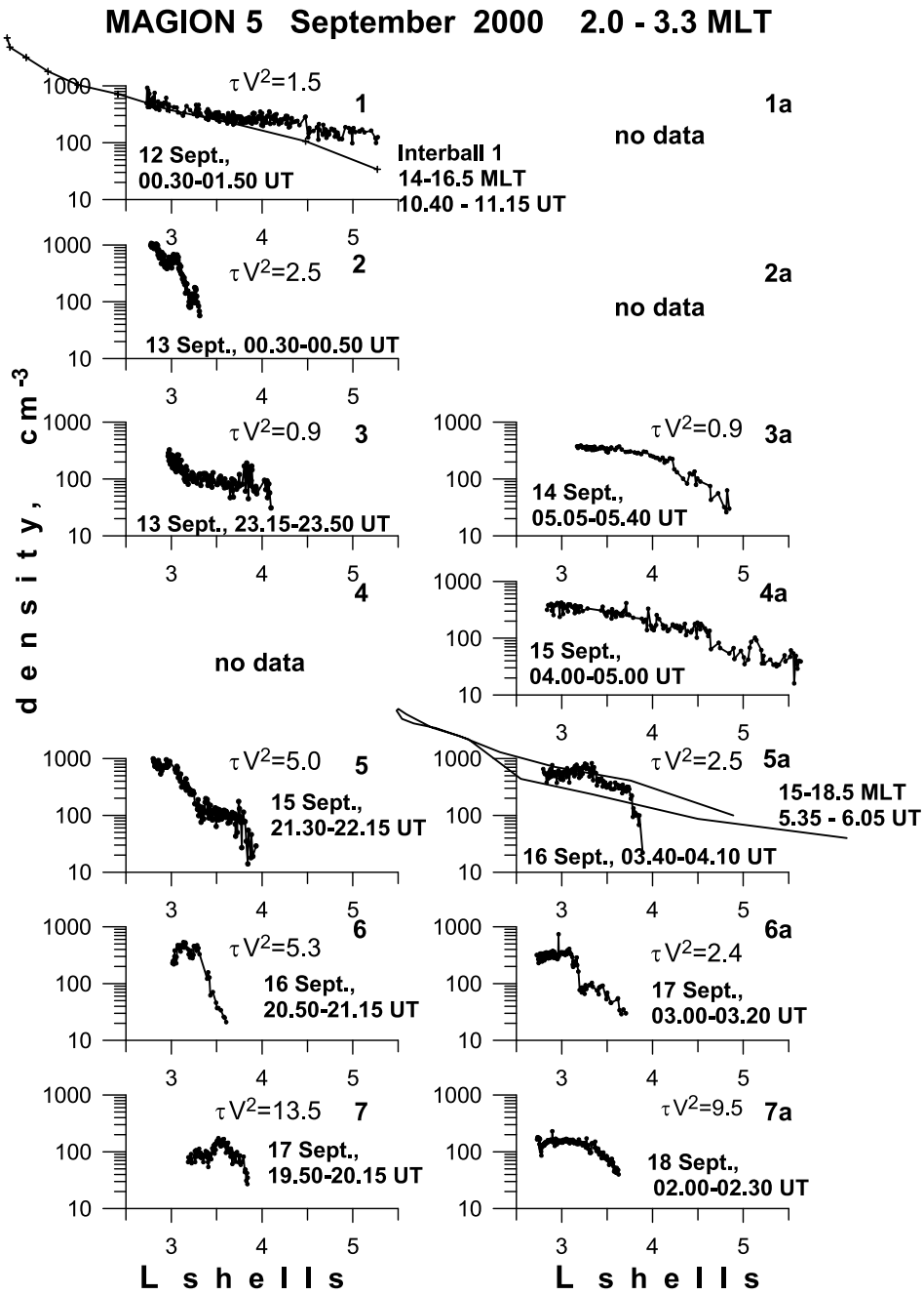
Fig. 3(a). Density versus L profiles measured at 2.0–3.3 MLT in a number of successive inbound plasmasphere passes during 12–18 September 2000. \rho V^2 values give the solar wind dynamic pressure measured by the ACE spacecraft and shifted to the Earth ( http://cdaweb.gsfc.nasa.gov/ ). In panels 1 and 5a Interball 1 measurements are shown for comparison.
