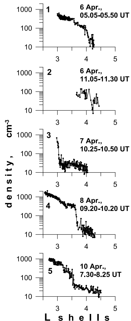
Fig. 7. Density versus L profiles measured at 8.3–9.1 MLT in a number of successive inbound plasmasphere passes in April 2001.
