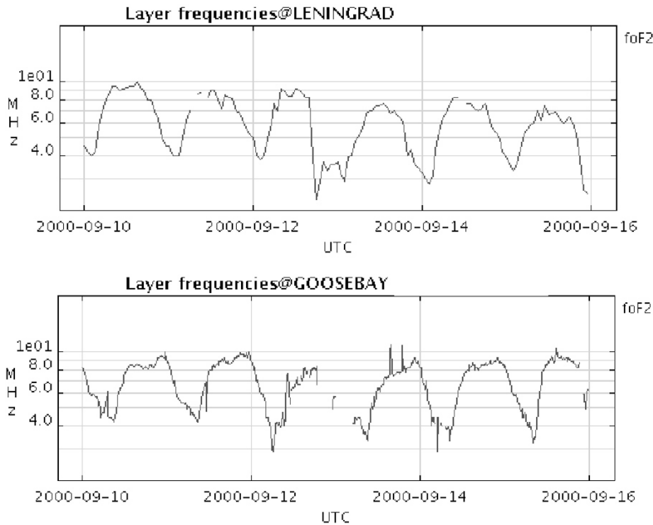
Fig. 4. Critical frequencies of ionospheric F2 layer provided by http://spidr.ngdc.noaa.gov/spidr/ .
