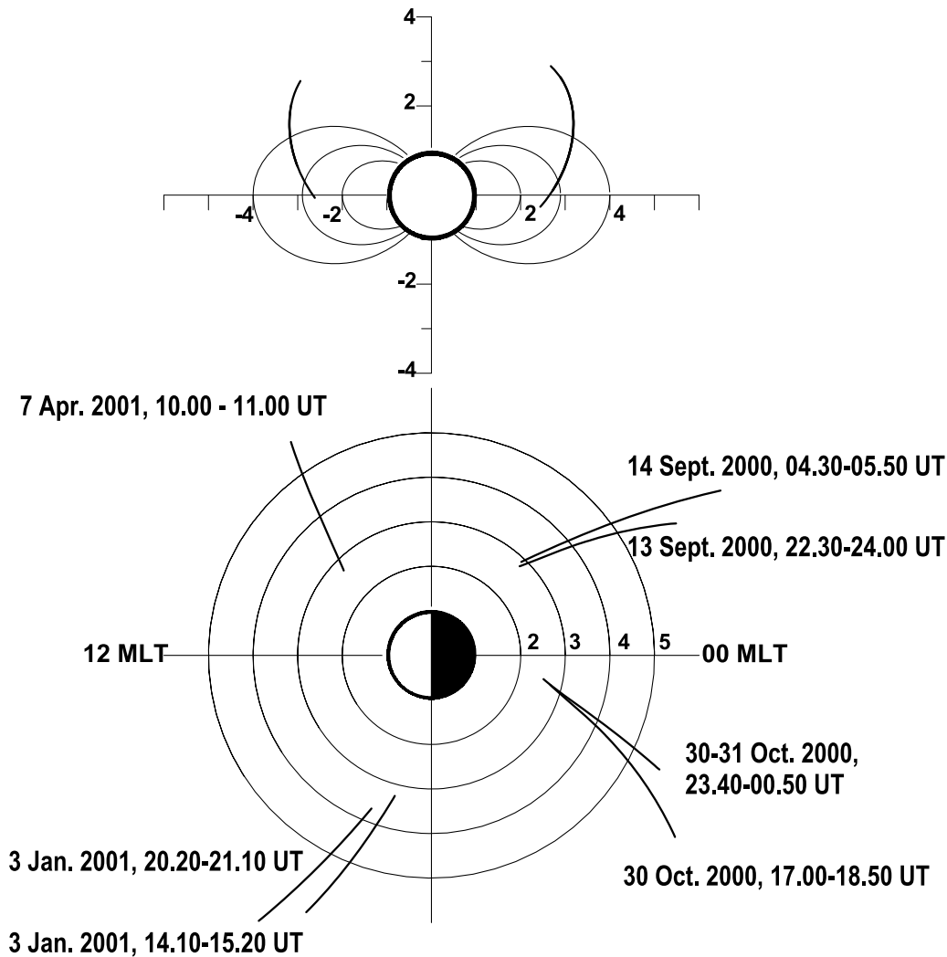
Fig. 1. Examples of MAGION 5 inbound trajectory parts in the inner magnetosphere. Meridian (upper) and equatorial (lower) projections. The axes are scaled by the Earth's radius ( R_E ).
