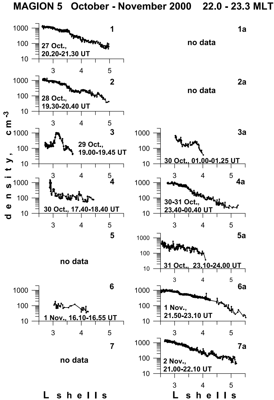
Fig. 2(a). Density versus L profiles measured at 22.0–23.3 MLT in a number of successive inbound plasmasphere passes during 27 October–2 November 2000.
