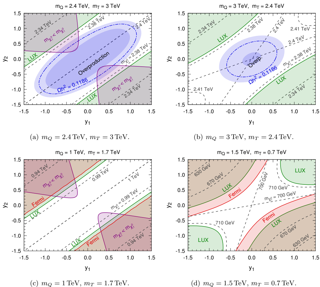
Figure 6. Constraints on the y_1 - y_2 plane for four sets of fixed m_Q and m_T as indicated. The legend for the lines and shadings are the same as in figure 5.
