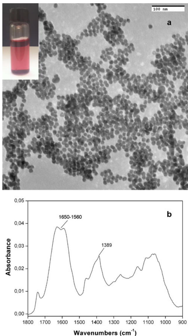
Fig. 2 a TEM micrograph and b FTIR spectrum of colloidal Au NPs used as dispersed phase
