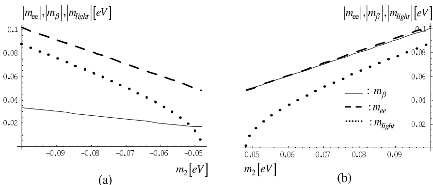
Figure 12. The |m_{ee}| , |m_\beta| and |m_{light}| as functions of m_2 from (5.47) in the case of \Delta m_{23}^2 < 0 and \delta = \frac{\pi}{2} . (a) m_2 \in (-0.1, -0.0482) eV, (b) m_2 \in (0.0482, 0.1) eV.
