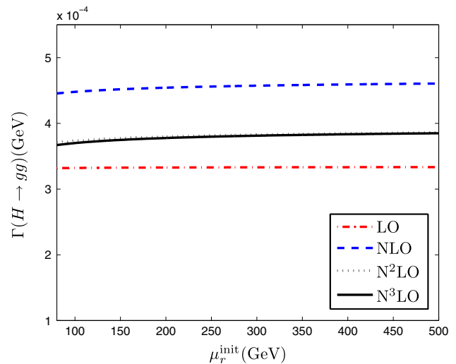
Fig. 6 Total decay width \Gamma(H \rightarrow gg) up to three-loop level after PMC scale setting versus the initial renormalization scale \mu_r^{\text{init}} . The dash-dot , dashed , dotted , and solid lines are for LO, NLO, N^2\text{LO} , and N^3\text{LO} estimations, respectively
