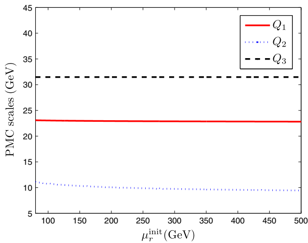
Fig. 4 The LO, NLO, and NNLO PMC scales Q_1 , Q_2 and Q_3 versus the initial renormalization scale \mu_r^{\text{init}} for the H \rightarrow gg process, which are shown by solid , dotted , and dashed lines, respectively. M_H = 126 GeV
