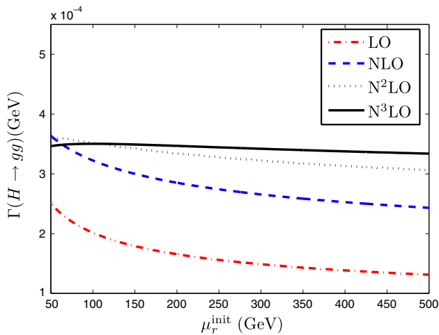
Fig. 5 Total decay width \Gamma(H \rightarrow gg) up to three-loop level under conventional scale setting versus the renormalization scale \mu_r \equiv \mu_r^{\text{init}} . The dash-dot , dashed , dotted and solid lines are for LO, NLO, N^2\text{LO} , and N^3\text{LO} estimations, respectively
