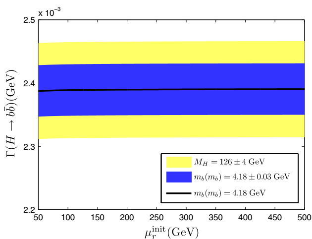
Fig. 7 Uncertainties for the decay width of H \rightarrow b\bar{b} up to four-loop level. Two shaded bands shows the uncertainties from M_H = 126 \pm 4 GeV and the \overline{\text{MS}} b -quark mass m_b(mb) = 4.18 \pm 0.03 GeV, respectively. The solid line is obtained by set the parameters to be their central values
