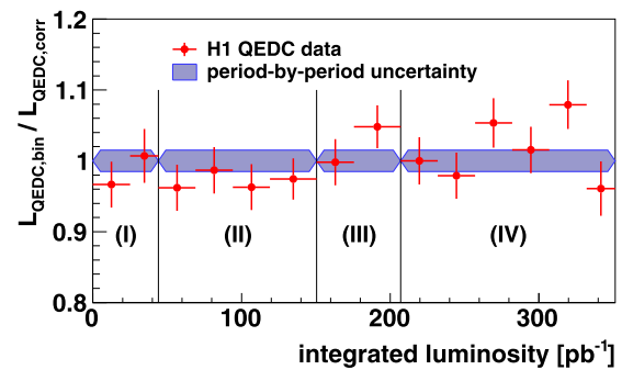
Fig. 7 Integrated luminosity measured from elastic QEDC events in bins of approximately 25 \text{ pb}^{-1} , divided by the integrated luminosity derived from the QEDC analysis on the full sample with time-dependent corrections applied. The statistical uncertainties of the binned QEDC analysis as well as the uncertainties of the time-dependent corrections, here applied to four data taking periods (I)–(IV), are indicated
