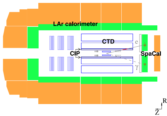
Fig. 1 Elastic QEDC candidate event observed in the H1 detector. The H1 detector components most relevant to this analysis are indicated. The approximate electron and photon candidate trajectories are shown
