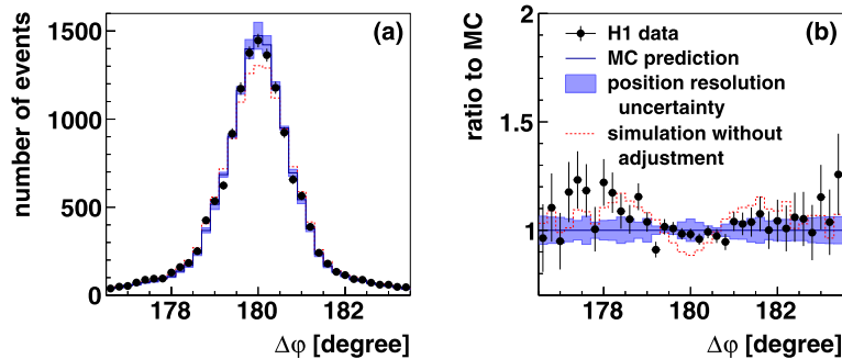
Fig. 4 Distributions of the difference in azimuth between the electron and the photon. In (a) the event counts are shown, whereas in (b) the ratio to the expectation is drawn. The data are shown as black dots with statistical uncertainties indicated as vertical bars . The simulation including background, normalised to the integrated luminosity as de-
