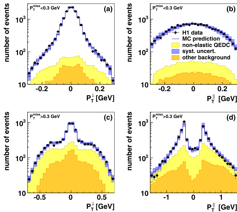
Fig. 5 Distributions of components of the photon plus electron transverse momentum sum, \vec{P}_T^{\text{sum}} : (a) and (c) the component perpendicular to the electron transverse momentum, (b) and (d) the component parallel to the electron transverse momentum. The upper row, (a) and (b) shows the distributions inside the analysis phase space, the lower row (c) and (d) shows the distributions for |P_T^{\text{miss}}| > 0.3 GeV. The
