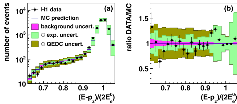
Fig. 6 Distribution of the variable (E - p_z)/2E_e^0 calculated from the sum of the electron and photon four-momenta. In (a) the event counts are shown, whereas in (b) the ratio of data to expectation is drawn. The data are shown as black dots with the statistical uncertainties indicated
