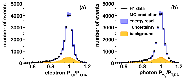
Fig. 3 Distributions of the ratio of measured to predicted transverse momentum for (a) electrons and (b) photons. The predicted transverse momentum P_{T,DA} is calculated using the double angle method. The data are shown as black dots . The simulation including background, normalised to the integrated luminosity as determined in this analysis,
