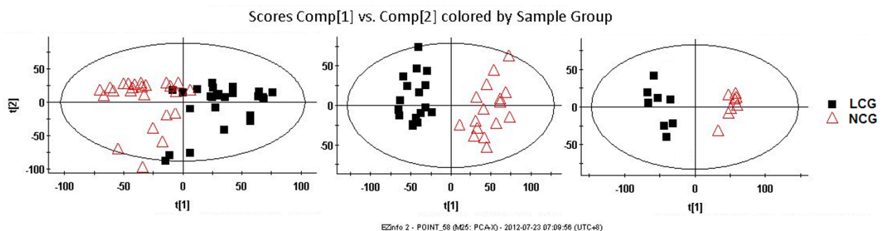
Figure 4 Principal component analysis (PCA) score plots of rats in the low-calcium group (LCG) and normal-calcium group (NCG). (A-C) Week 2, n = 48 (for two components, R^2Y = 45.0\% , Q^2 = 24.1\% ); week 4, n = 32 (for three components R^2Y = 54.6\% , Q^2 = 27.6\% ) and week 9, n = 16 (for three components R^2Y = 58.3\% , Q^2 = 32.1\% ). The R^2Y value represents the goodness of fit of the model, and the Q^2 value represents the predictability of the models. LCG rats are indicated by black squares and NCG rats by red triangles. Each data point represents one subject. Comp, component. t[1] , component 1; t[2] , component 2.
