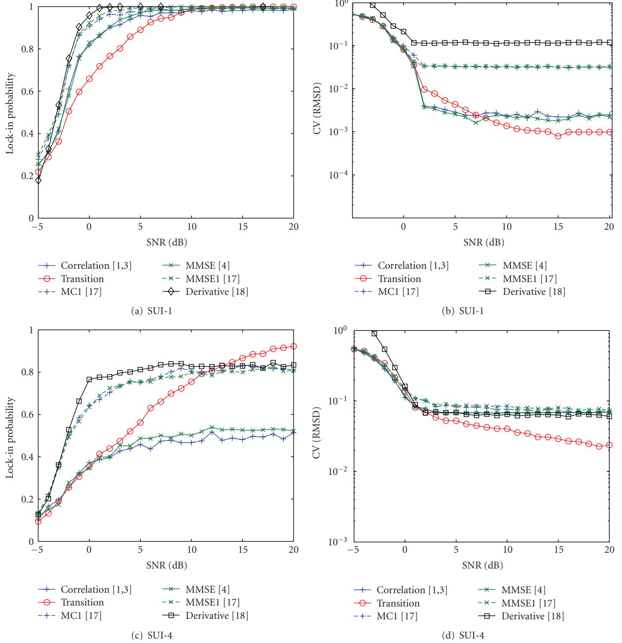
FIGURE 3: Simulations' results for CP-OFDM transmission.
