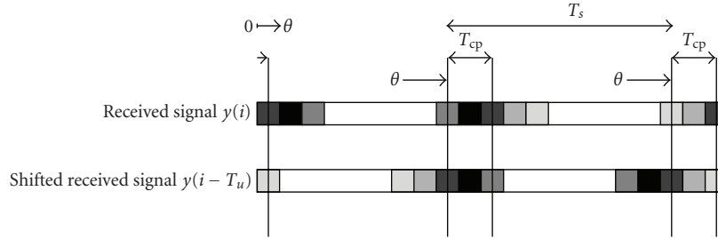
FIGURE 2: Windows used for timing offset estimation.
