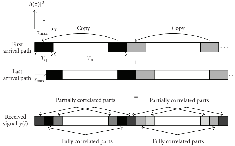
FIGURE 1: Effect of the multipath replicas on the transmitted signal.
