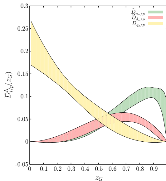
Fig. 2 Spectator-fragmentation functions \tilde{D}_{i/p}^\Lambda(z_G) for valence u (green), d (red) and sea (yellow) quarks extracted from the fit of Ref. [8]. The bands represent the propagation of experimental uncertainties according to the \Delta\chi^2 = 1 criterion
