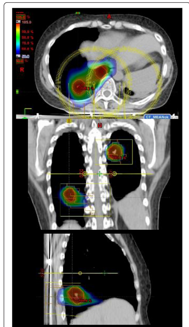
Figure 1 An example of dose distribution for a 3-lesion patient. The 50% isodose distribution is pointed out showing a qualitative overview of the target coverage and dose fall down outside the PTV.
