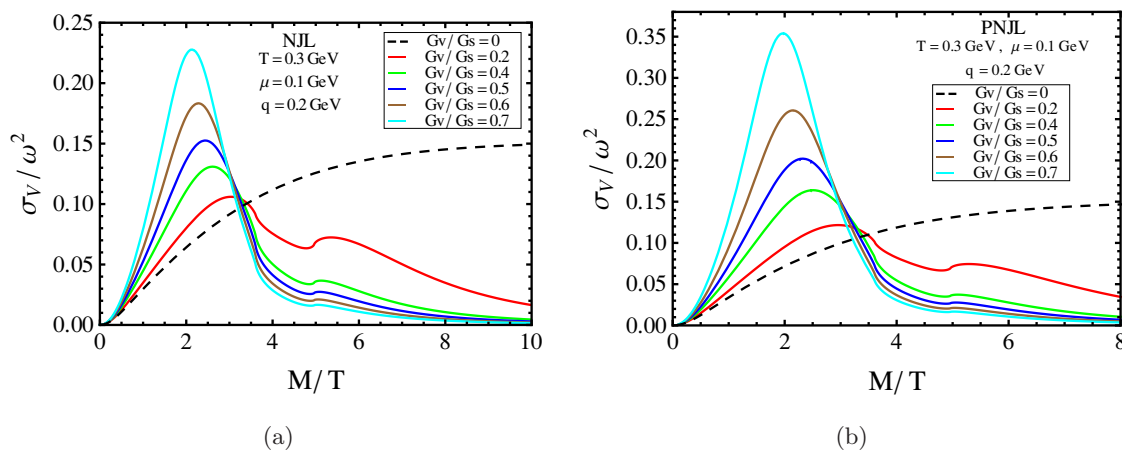
Figure 12. Scaled spectral function as a function of M/T for (a) NJL and (b) PNJL model with T = 300 MeV, \mu = 100 MeV, q = 200 MeV and a set of values of G_V/G_S = 0, 0.2, 0.4, 0.5, 0.6 and 0.7 .
