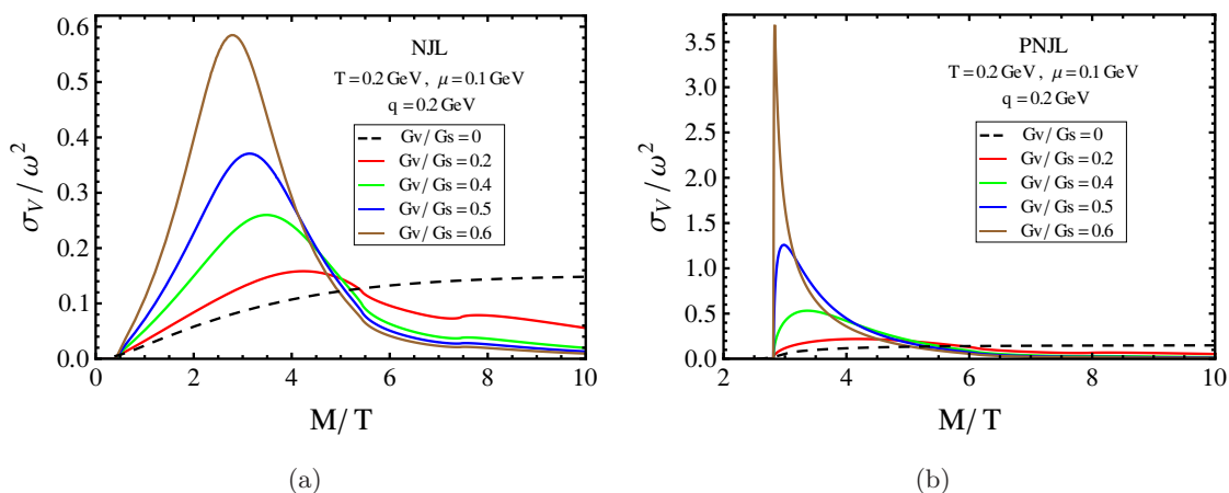
Figure 11. Scaled spectral function as a function of M/T for (a) NJL and (b) PNJL model with T = 200 MeV, \mu = 100 MeV, q = 200 MeV and a set of values of G_V/G_S = 0, 0.2, 0.4, 0.5 and 0.6 .
