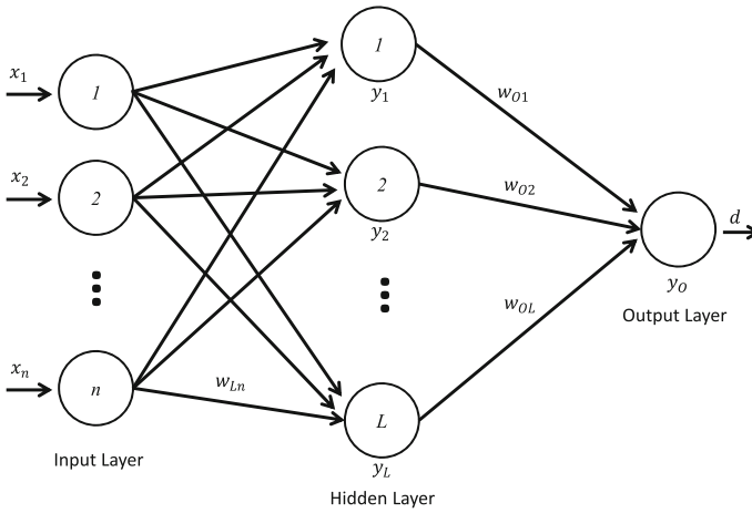
Fig. 2 A simple three-layer MLP
