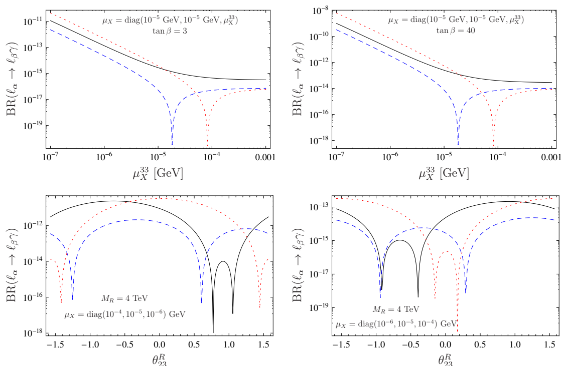
Figure 7. Dependence of \ell_\alpha \rightarrow \ell_\beta \gamma on \mu_X^{33} and \theta_{23}^R . The lines correspond to \text{BR}(\mu \rightarrow e \gamma) (black), \text{BR}(\tau \rightarrow e \gamma) (blue dashed) and \text{BR}(\tau \rightarrow \mu \gamma) (red dotted).
