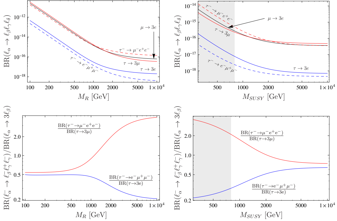
Figure 5. Branching ratios for \tau decays as a function of M_R and M_{SUSY} . In the upper two plots the lines correspond to BR(\mu \rightarrow 3e) (black solid), BR(\tau \rightarrow 3e) (blue solid), BR(\tau \rightarrow 3\mu) (red solid), BR(\tau^- \rightarrow e^- \mu^+ \mu^-) (blue dashed) and BR(\tau^- \rightarrow \mu^- e^+ e^-) (red dashed). The gray area roughly corresponds to the parameter space excluded by the LHC experiments.
