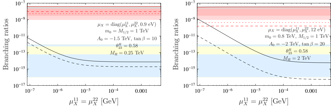
Figure 6. \mu - and \tau -observables as a function of \mu_X . The underlying parameters are given in the plots. The lines correspond to BR(\tau \rightarrow \mu\gamma) (full red), BR(\tau \rightarrow 3\mu) (dashed red), BR(\tau^- \rightarrow \mu^- e^+ e^-) (dotted red), BR(\mu \rightarrow e\gamma) (full black) and BR(\mu \rightarrow 3e) (dashed black). The light gray, red, yellow and blue bands show the expected future reach of the dedicated experiments to \tau \rightarrow \mu\gamma , \tau \rightarrow 3\mu , \mu \rightarrow e\gamma and \mu \rightarrow 3e as given in table 1.
