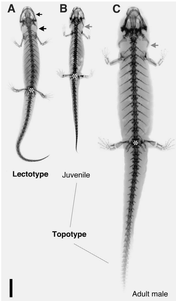
Fig. 4. X-ray photographs of the lectotype (A: ZMB 34087) and topotypes of a juvenile (B: CIB GX20081029) and an adult male (C: CIB GX20081006) of Pachytriton labiatus . Large arrows showing the tip of epibranchials (black: nearly straight; grey: curving as if wrapping the neck). A small arrow showing the tip of maxilla oriented angular to the body axis. Asterisks showing the sacrum vertebrae. Scale bar = 10 mm.
