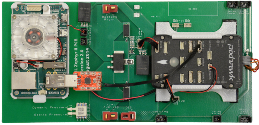
Fig. 2. ARSENL’s custom printed circuit board for ZephyrII , providing power distribution, airspeed and power sensing, wiring interfaces, and 3D-printed mounts for autopilot and autonomy computer modules.
