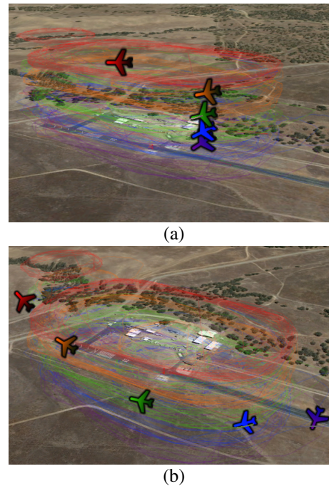
Fig. 9. Live-fly examples of leader-follower of two basic configurations, where (a) all followers trail a single leader, or (b) followers are in a (close) trail formation
