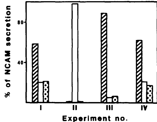
Fig.3. Secretion of NCAM. In four separate experiments a neuronal cell culture was labelled for 15 min with [ 35 S]methionine followed by three successive chase periods of 15 min. NCAM was immunisolated from each of the three chase media and secretion determined setting the total amount of NCAM dpm (~500) isolated from the three chase media to 100%. (Hatched bars) Fraction secreted in the period 15-30 min after the start of synthesis; (unfilled bars) 30-45 min after start of synthesis; (dotted bars) 45-60 min.
