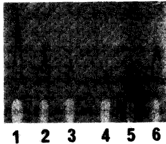
Fig.1. Demonstration of PSA residues in soluble NCAM. Rocket immunoelectrophoresis against polyclonal anti-NCAM of an NCAM standard (32 µg/ml) in dilutions 1:1, 1:2, 1:4 and 1:8 (wells 1-4) and soluble NCAM with anti-PSA (well 5) or preimmune horse serum (well 6).
