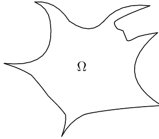
Fig. 1. A quasi-convex domain.
