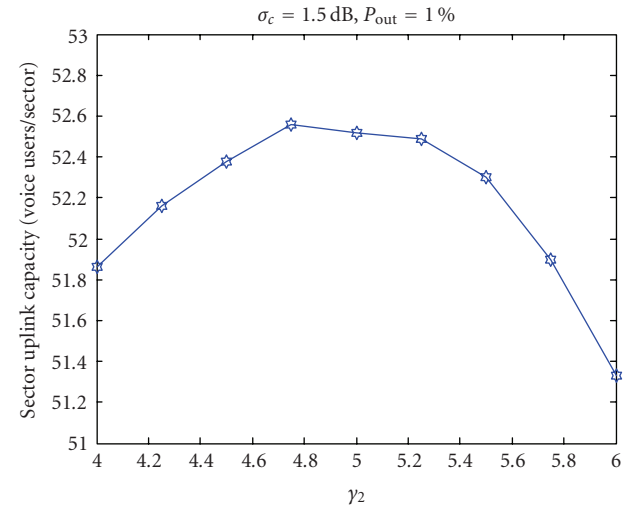
FIGURE 13: Effect of the propagation exponent \gamma_2 on the sector uplink capacity.
