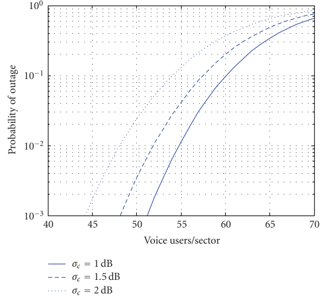
FIGURE 4: Outage probability of the sector for voice users only.
