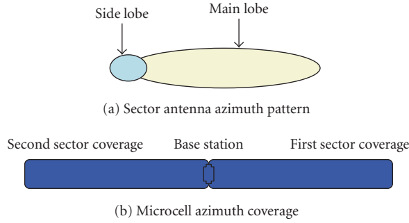
FIGURE 1: The sector and microcell coverage.
