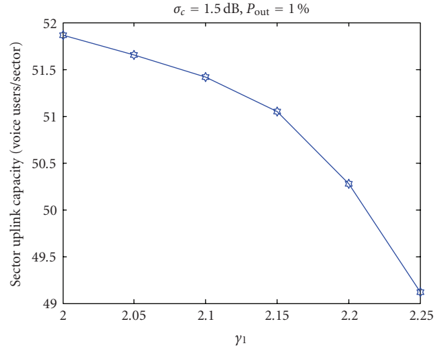
FIGURE 12: Effect of the propagation exponent \gamma_1 on the sector uplink capacity.
