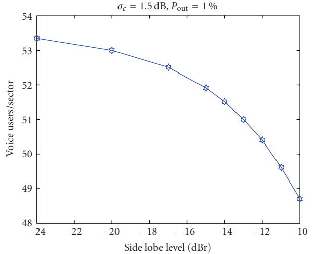
FIGURE 9: Effect of the antenna sidelobe level on the sector uplink capacity.
