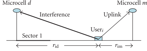
FIGURE 3: Schematic diagram of base stations and mobiles for high-way microcells.
