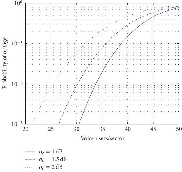
FIGURE 6: Outage probability of the sector for mixed voice and data users.
