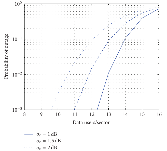
FIGURE 5: Outage probability of the sector for data users only.
