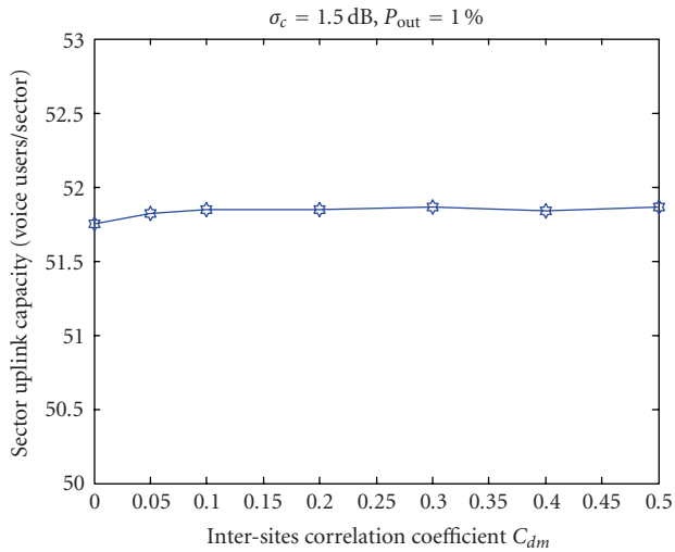
FIGURE 11: Effect of the inter-sites correlation coefficient on the sector uplink capacity.
