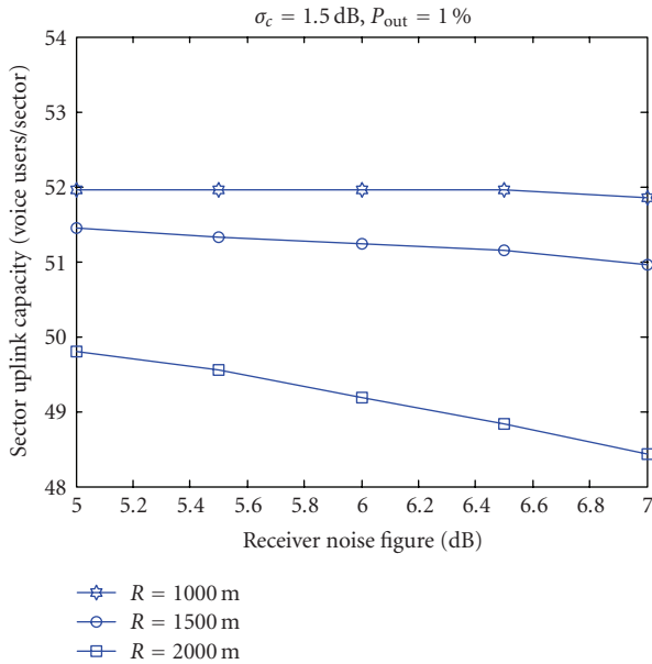
FIGURE 14: Effect of the base station receiver noise figure on the sector uplink capacity.
