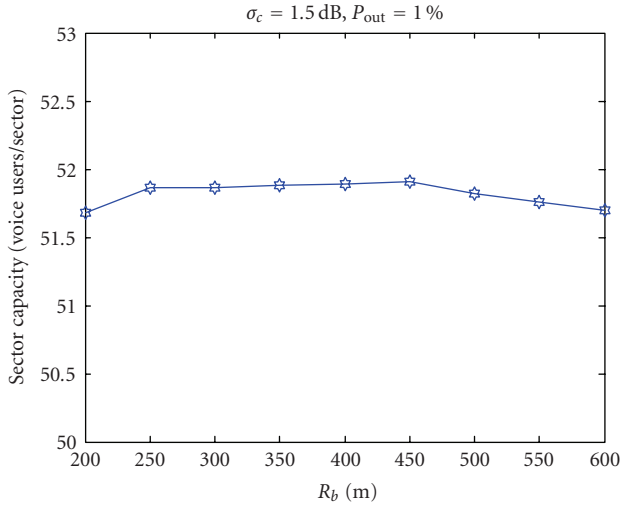
FIGURE 10: Effect of the break point distance R_b on the sector uplink capacity.
