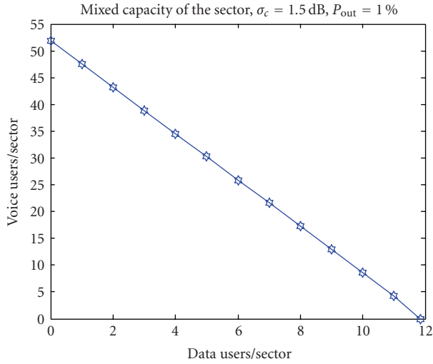
FIGURE 7: Mixed capacity of the sector.
