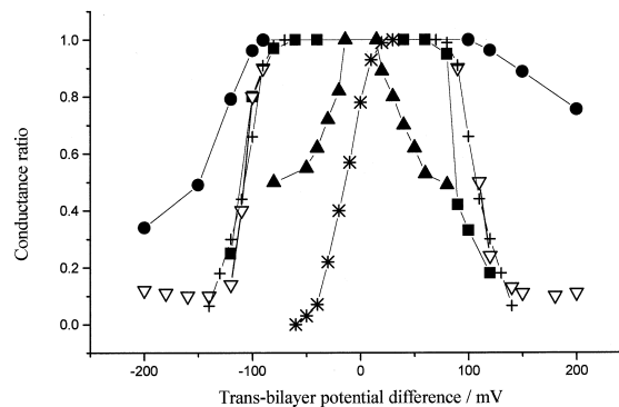
Fig. 2. The voltage dependence of five unrelated \beta -barrel pores. The graph shows the ratio of conductance (R) at each voltage compared to the conductance measured at a low voltage that does not induce gating. All data from planar lipid bilayer experiments replotted from original references. ●, \alpha -toxin in diphytanoyl-phosphatidylcholine bilayer, 100 mM KCl, 5 mM HEPES, pH 7.4 [44]; ■, aerolysin in soybean lecithin bilayer, 1 M NaCl, 10 mM HEPES, 1 mM EDTA, pH 7.4 [38]; ▲, Paramaecium mitochondrial porin in 0.5 M KCl pH 7.2 [45]; ▽, E. coli PhoE in 1 M NaCl, 10 mM MgCl 2 , 10 mM Tris-HCl pH 7.4; soybean lecithin bilayer [28]; +, Neisseria gonorrhoeae porin in phosphatidylethanolamine, phosphatidylcholine, cholesterol bilayer, 0.1 M NaCl, 10 mM HEPES pH 7.4 [13]. *, Voltage dependence of squid giant axon sodium channels for comparison [1].
