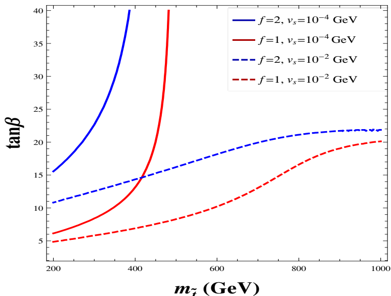
Figure 2. Mass-contours for the lightest Higgs boson with m_h = 125 GeV in the m_{\tilde{t}}\text{-tan}\beta plane for large values of f and \lambda_T = 0.5 .
