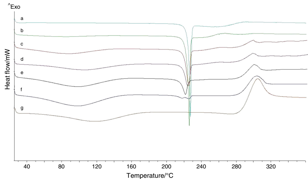
Fig. 5 DSC scans of: (a) hydrocortisone, (g) chitosan and their mixtures at drug/excipient ratios: (b) 9:1, (c) 7:3, (d) 1:1, (e) 3:7, (f) 1:9
