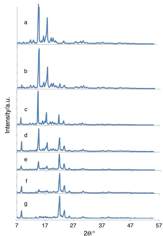
Fig. 11 Diffraction patterns of: (a) hydrocortisone, (g) magnesium stearate and their mixtures at drug/excipient ratios: (b) 9:1, (c) 7:3, (d) 1:1, (e) 3:7, (f) 1:9
