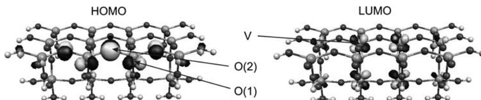
Fig. 9 The character of HOMO and LUMO orbitals for the V_{16}O_{52}H_{24} cluster modeling the V_2O_5(100) surface
