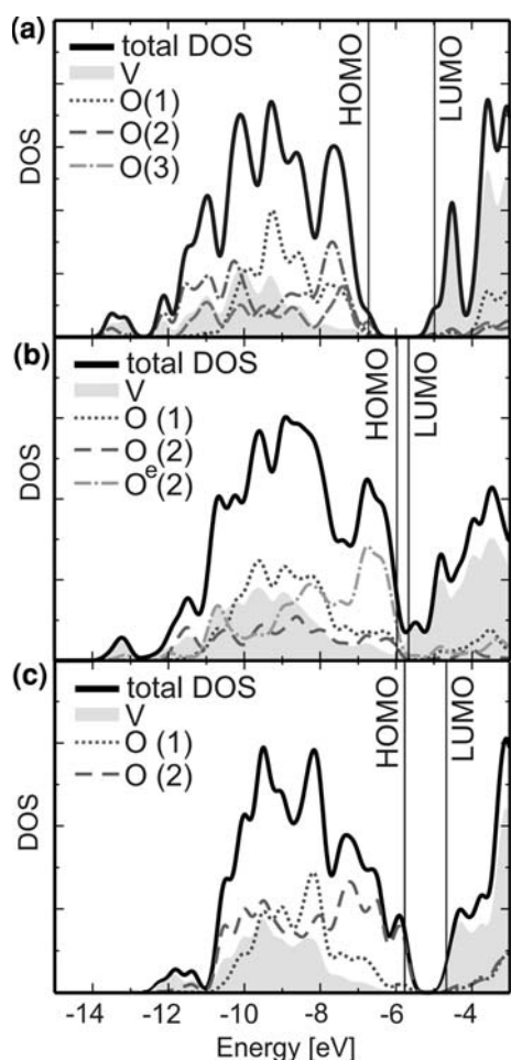
Fig. 3 DOS and pDOS plots for the valence region for the a V_2O_5(010) surface obtained with the V_{10}O_{31}H_{12} cluster, b V_2O_5(001) surface obtained with the V_{21}O_{65}H_{25} cluster and c V_2O_5(100) surface obtained with the V_{16}O_{52}H_{24} cluster
