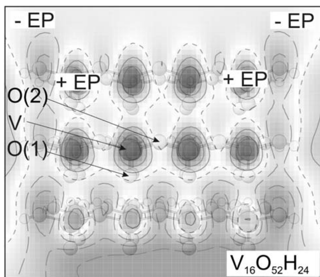
Fig. 8 The electrostatic potential map calculated at the distance of 2 Å above the V_2O_5(100) surface—projection from the above. Plot is obtained for V_{16}O_{52}H_{24} cluster. The “+EP” and “−EP” denote positive and negative values of EP, respectively
