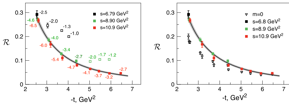
Fig. 3 Left the ratio \mathcal{R} as a function of t . The corresponding values of u are shown by the numbers next to the symbols. The open squares mark out the points with -u < 2.5 \text{ GeV}^2 . The solid line represents the empirical fit of Eq. (77), the gray bands show the 99 % confidence
